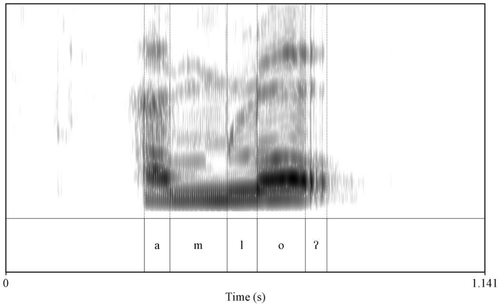
Figure 16: Spectrogram of amlo /àmló/ ‘heart’ (female speaker). This illustrates the word-end glottalisation, represented by [ʔ], that sometimes accompanies word-final H tones.
