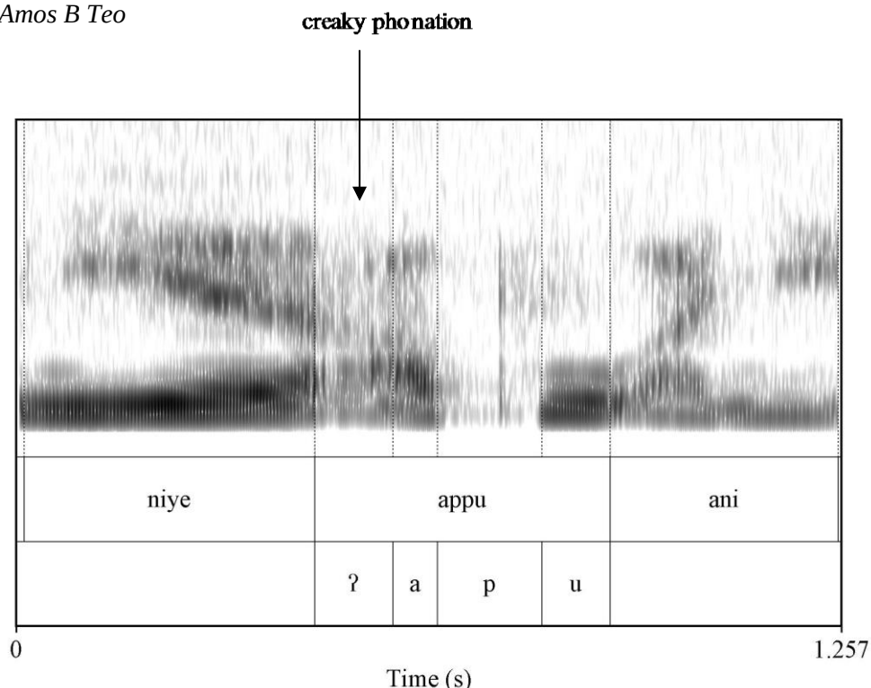
Figure 7: Spectrogram of niye appu [aɪ puɪ] ani ‘I have a son’ (female speaker)
