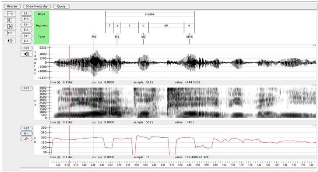
Figure 3: Sample annotation of atoque [a˩to˩q˥e˩] ‘lizard’ using the program Emu Labeler. From top to bottom, we have the three annotated tiers: Word, Segment and Tone; an acoustic waveform of the utterance; a wideband spectrogram and the pitch trace. In the Tone tier, ‘M’ marks M tone on vocalic segments within the investigated word, with the numbers 1, 2, 3 marking their position from the start of the word, and ‘%’ marking the tone on the last syllable of the word. ‘M0’ marks M tone in the part of the carrier phrase immediately preceding the investigated word.
