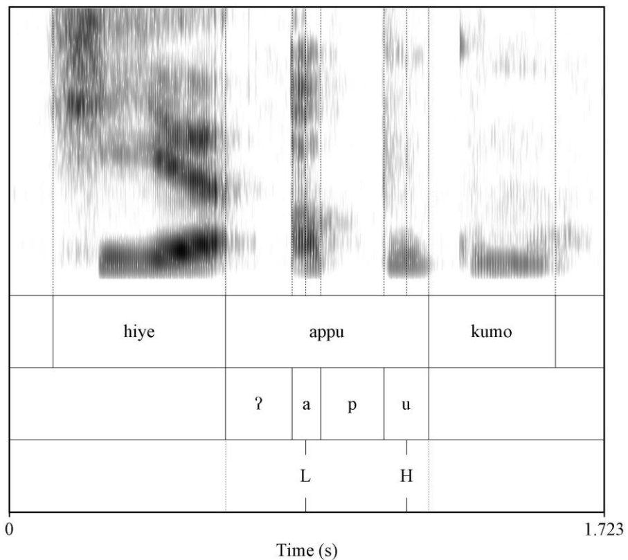
Figure 6: Spectrogram of hiye appu [ʔaɭ puɭ] kumo ‘This is not a son’ (male speaker)
